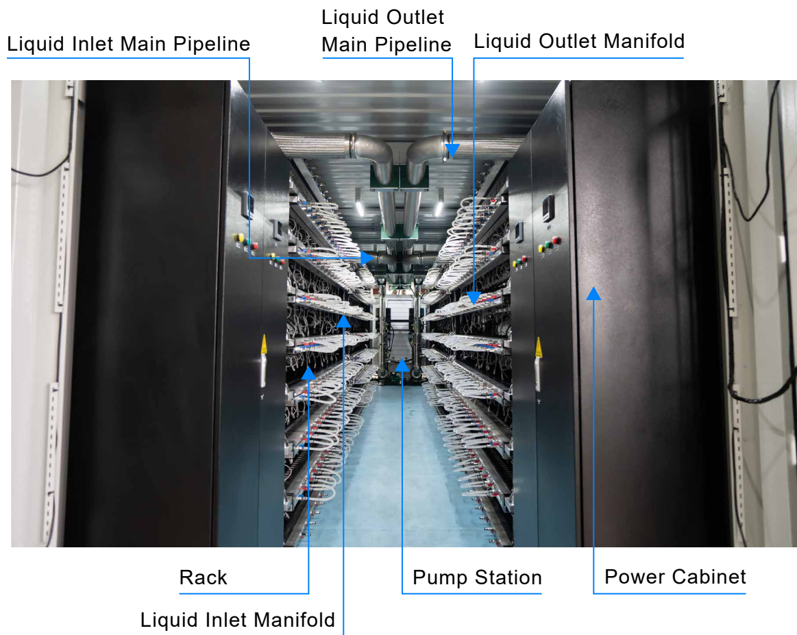
Figure 3-1-3 Container Internal Layout
