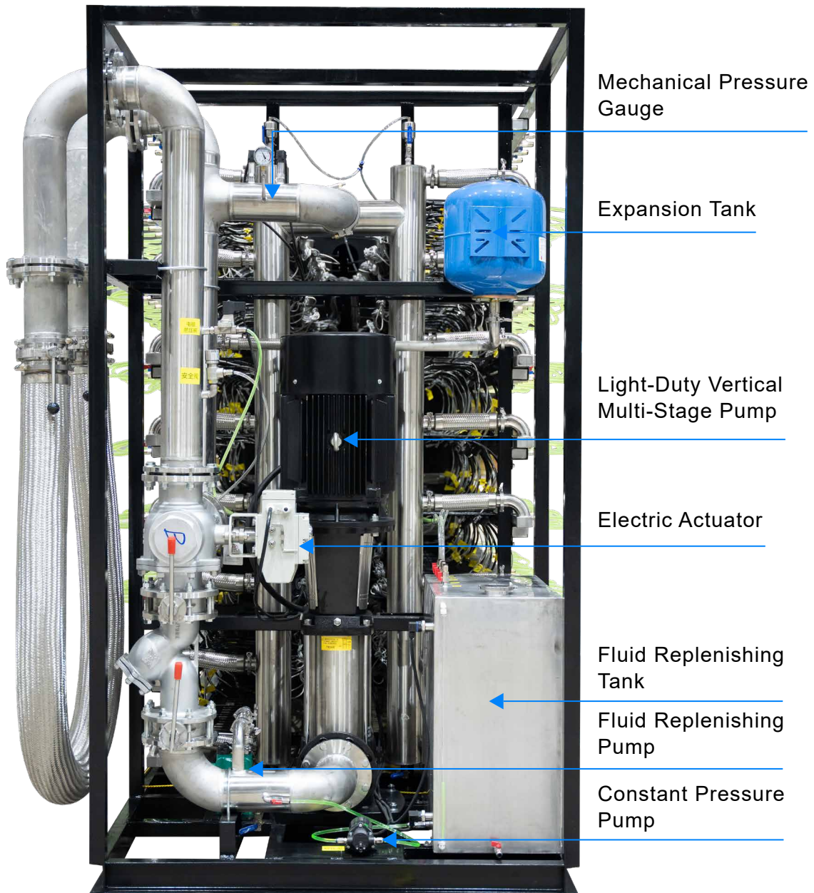
Figure 3-1-4 Components of the pump station
