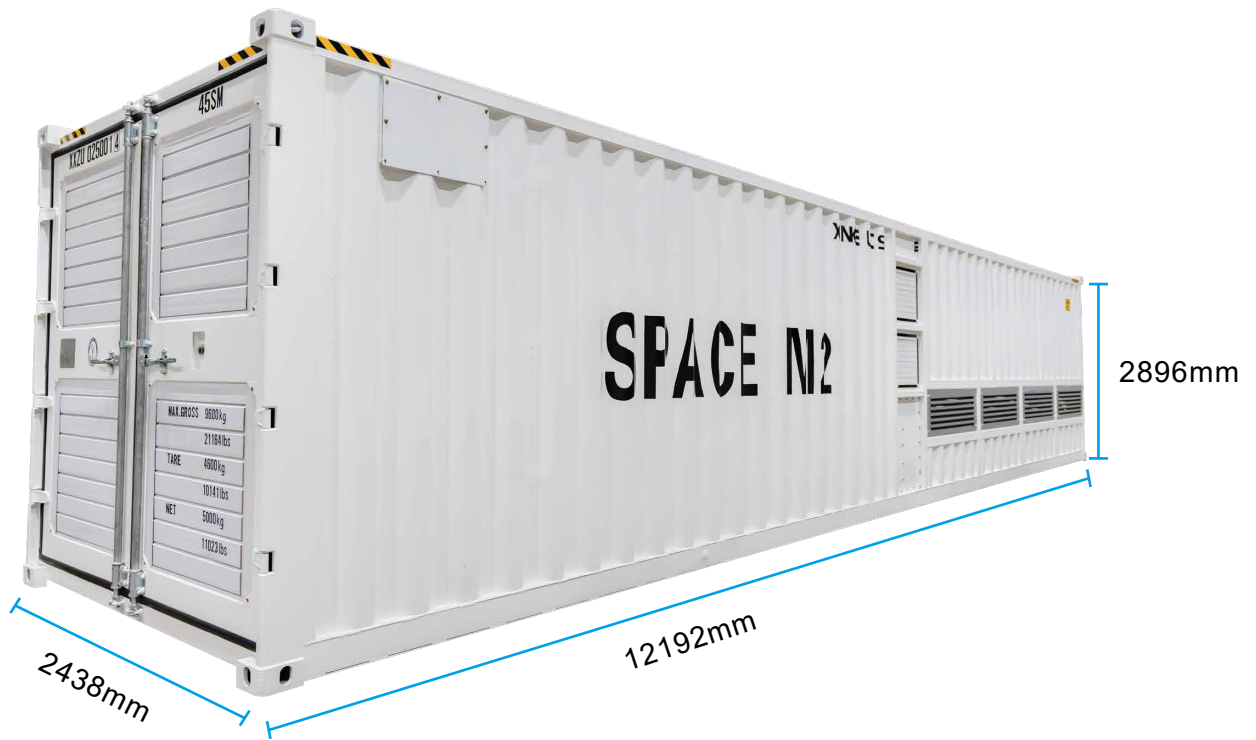
Figure 3-1-2 Container Dimensions
