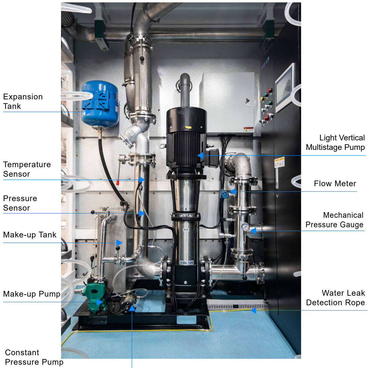
Figure 3-1-4 Container Pump Station Components
