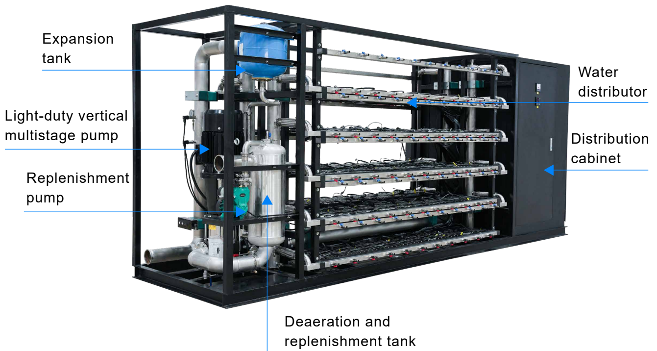
Figure 3-1-3 Internal Layout of the Rack
