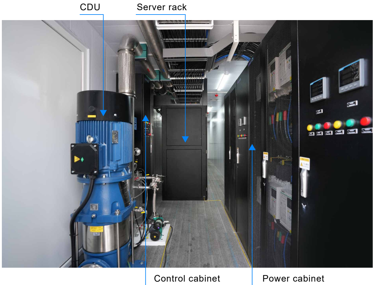
Figure 3-1-3 Interior layout of the container
