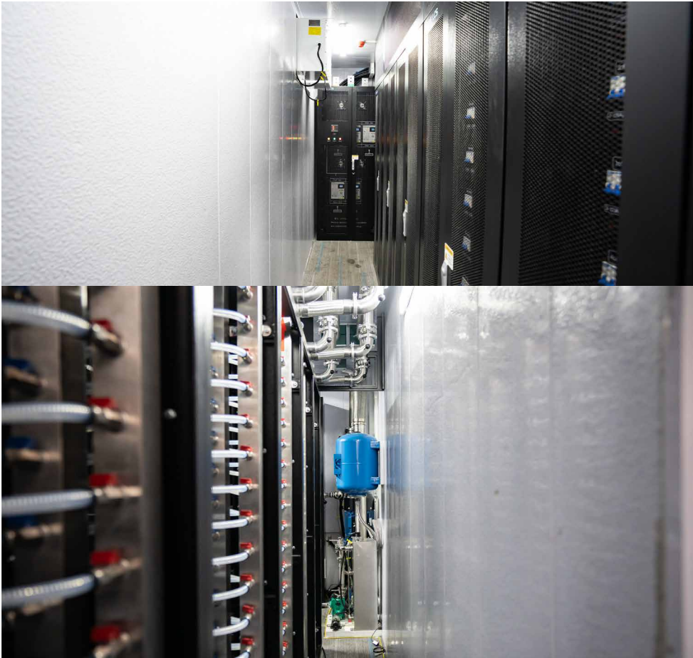
Figure 3-1-3 Interior layout of the container
