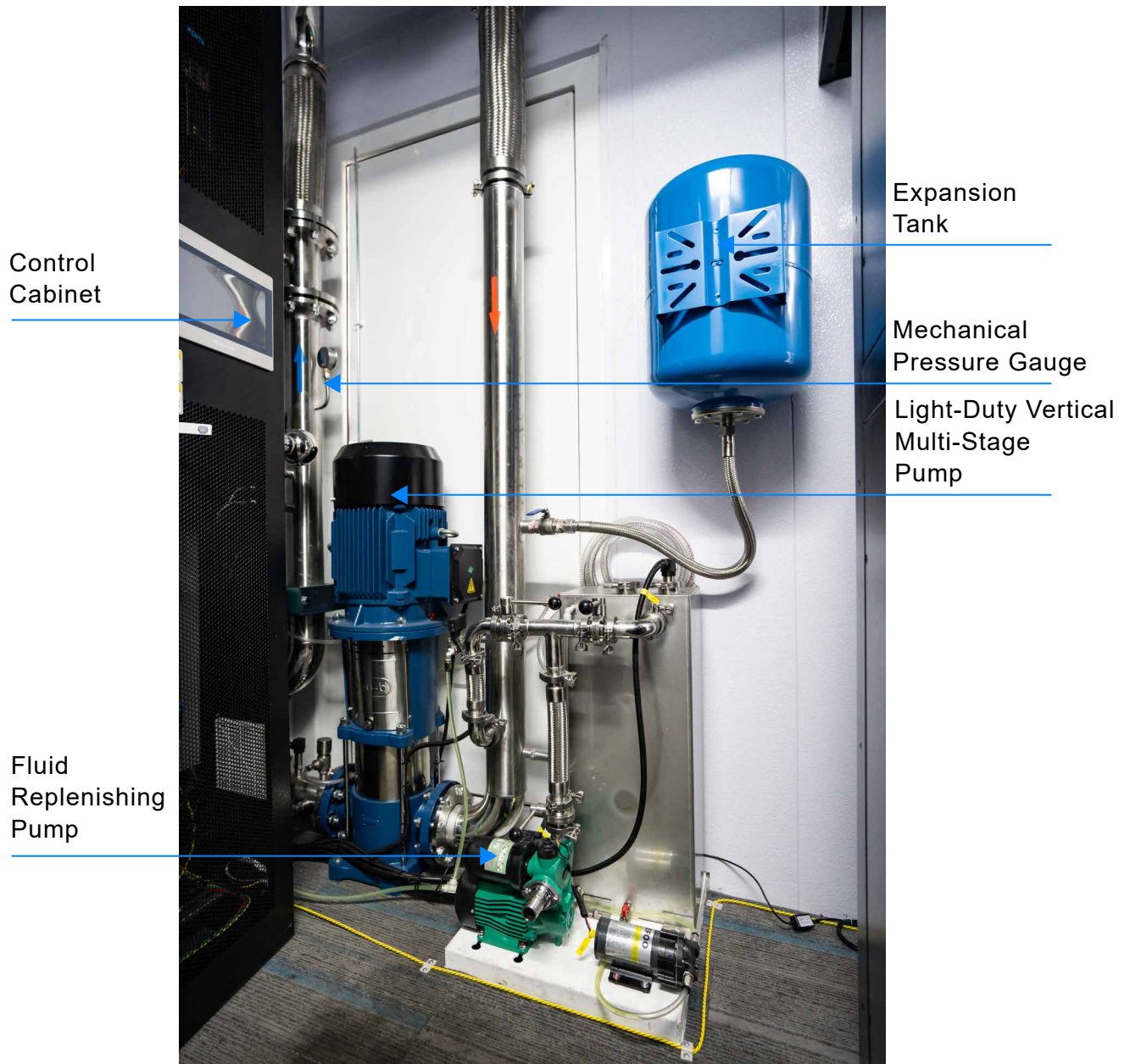
Figure 3-1-4 Components of the pump station
